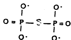
Thiobisphosphonate
